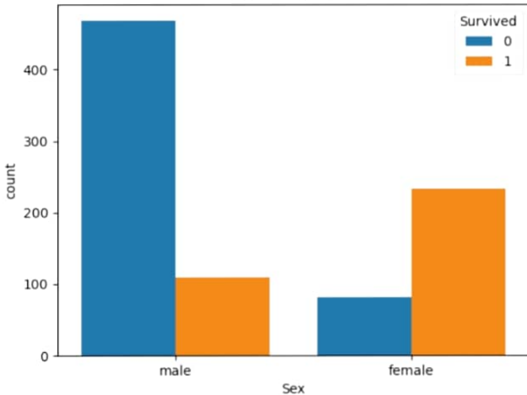
Survival by Gender
